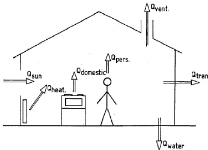
Figure 2. Schematic energy balance of a building. 3
